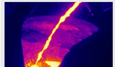
Measurement of casting stream during casting into a mold
