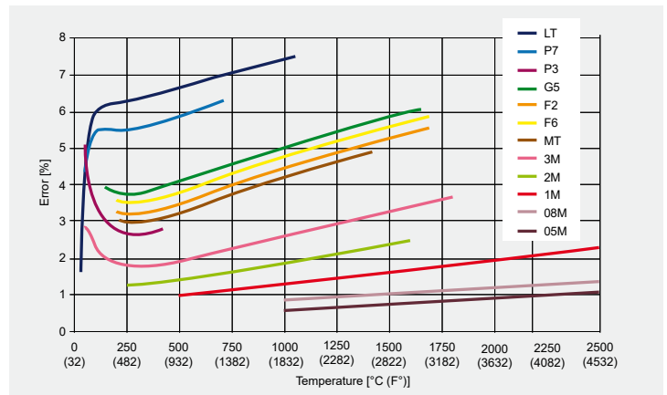
Measuring error in the case of emissivity wrongly adjusted by 10% as a function of the wavelength and object temperature (LT: 8–14 μm; P7: 7.9 μm; P3: 3.43 μm; G5: 5 μm; MT: 3.9 μm; F2: 4.24 μm; F6: 4.64 μm; 3M: 2.3 μm; 2M: 1.6 μm; 1M: 1.0 μm; 08M: 800nm; 05M: 525 nm.
